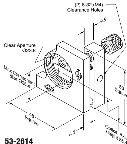
53-2614 Precise™ Thin Optic Mount, 1 inch
