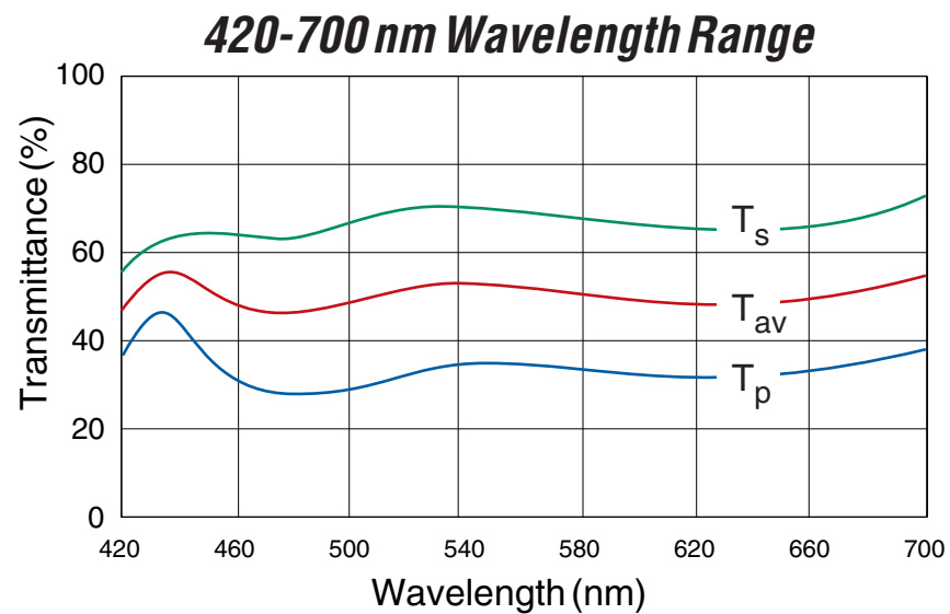
Broadband Beamsplitter Coating
